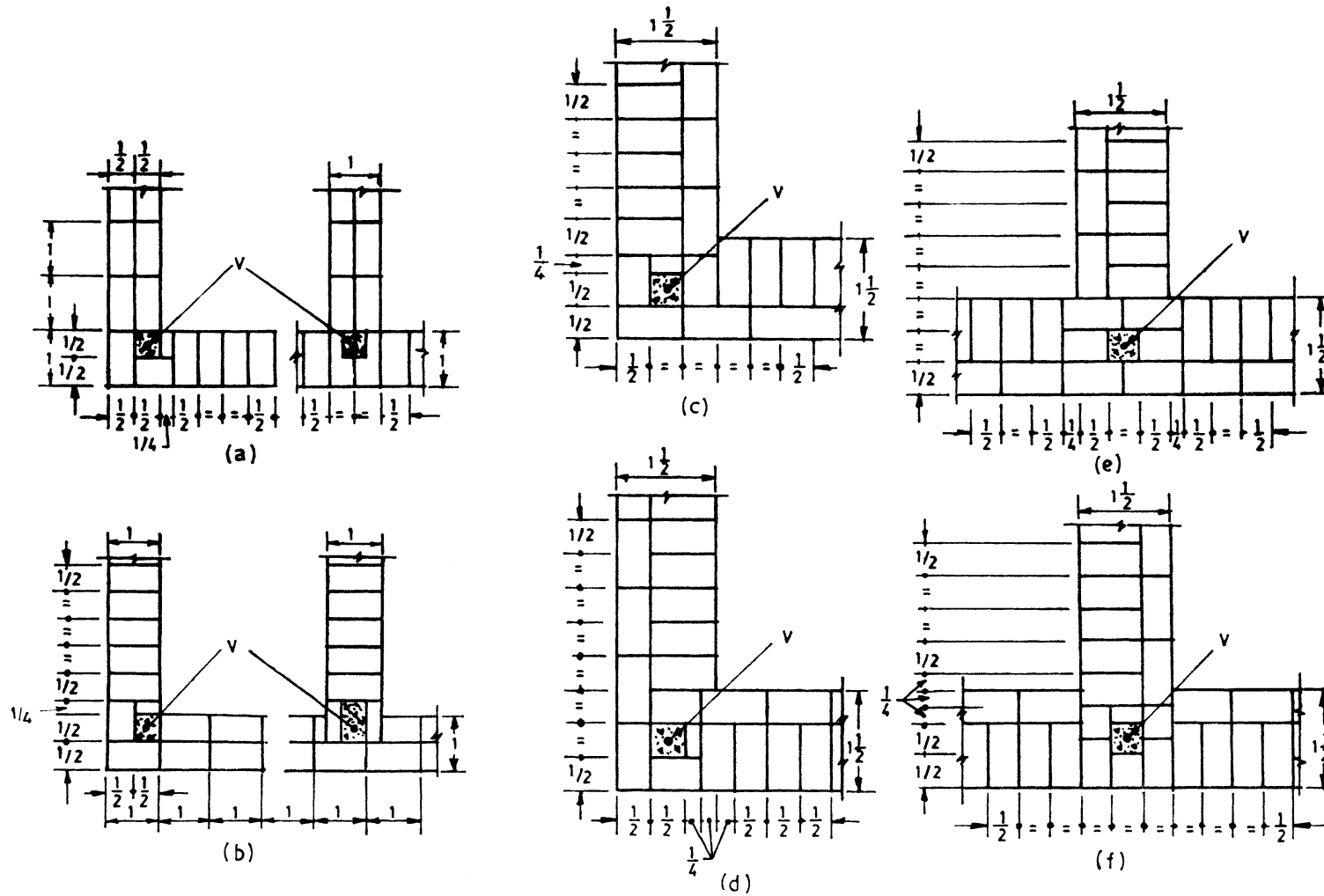
1 — One-brick length, \frac{1}{2} — Half-brick length, V — Vertical steel bar with mortar/concrete filling in pocket. (a) and (b) — Alternate courses in one brick wall. (c) and (d) Alternate courses at corner junction of 1\frac{1}{2} -brick wall. (e) and (f) Alternate courses at T-junction of 1\frac{1}{2} -brick wall.
