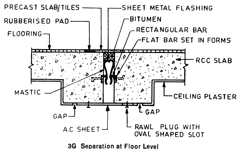
FIG. 3 TYPICAL DETAILS OF SEPARATION OR CRUMPLE SECTION
