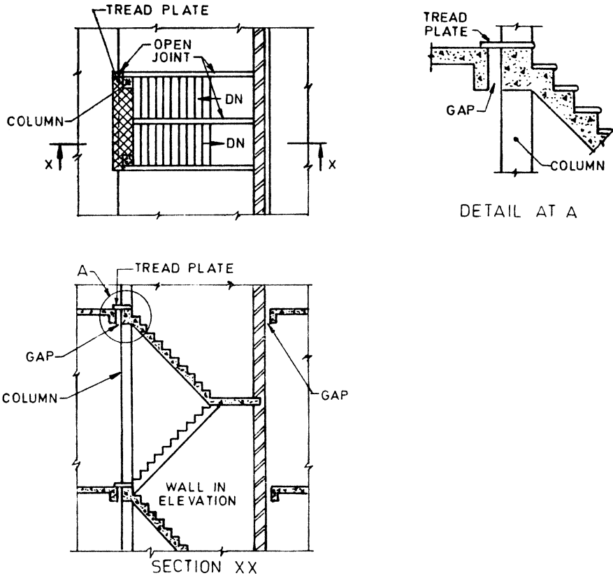
FIG. 4 SEPARATED STAIRCASE
